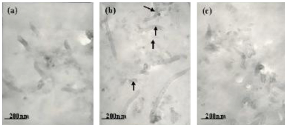
Fig. 4. TEM images of MWCNT/PVDF nanocomposites with aspect ratios of (a) 62, (b) 116 and (c) 437 (Reproduced from Yao et al. by permission of American Institute of Physics [63].).
